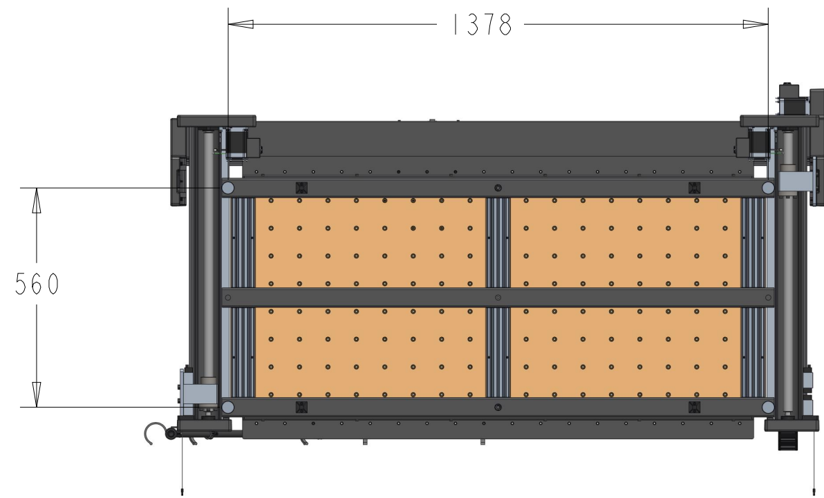
Leveling foot locations
